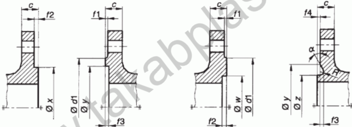
Type E: Spigot
