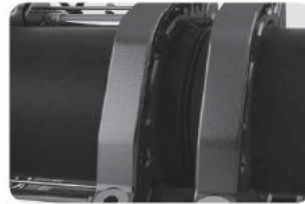
5. remove heater plate , close clamps to bring bead up .
